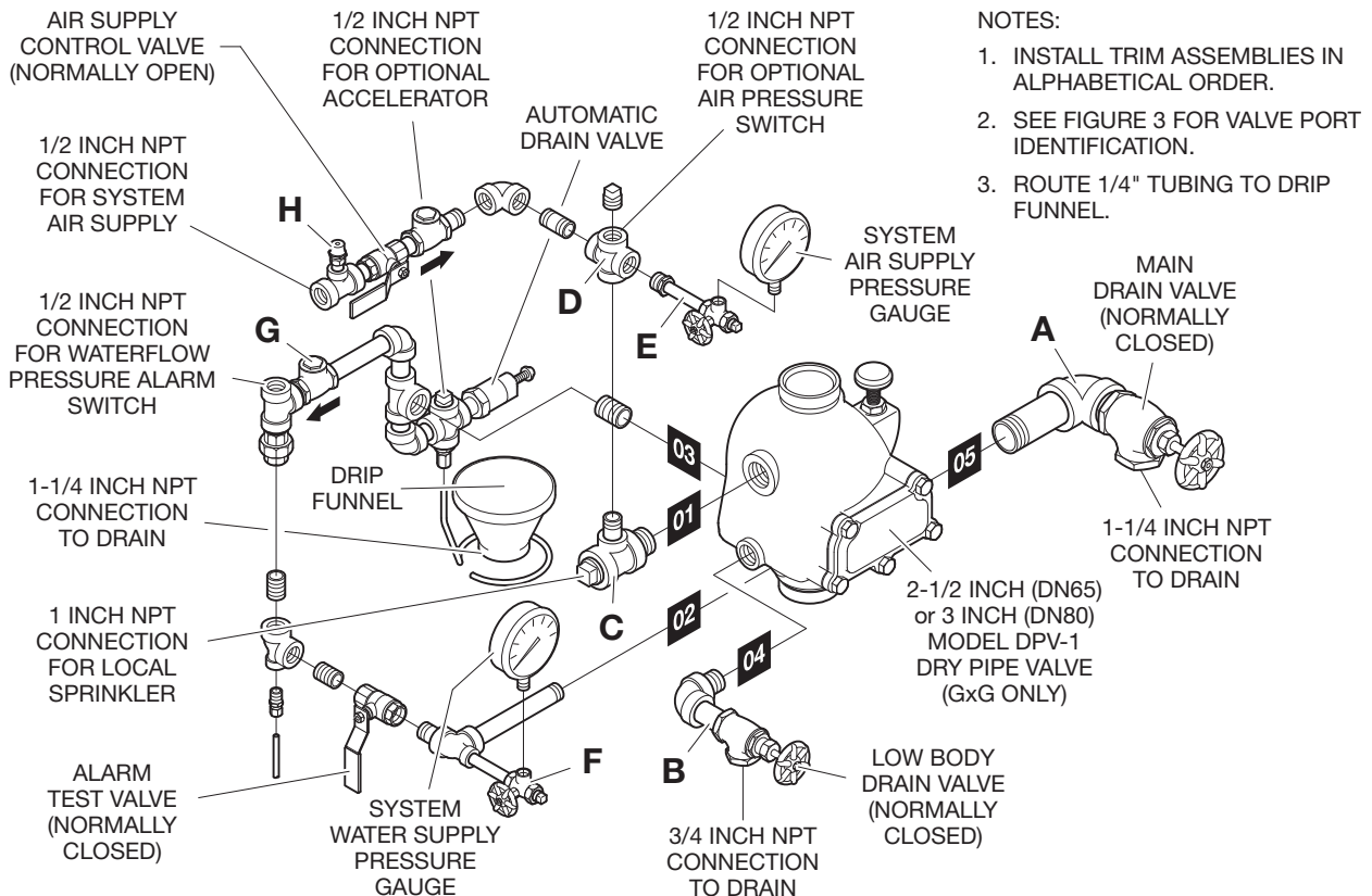
FIGURE 4 - PART 2 OF 3 2-1/2 AND 3 INCH (DN65 AND DN80) MODEL DPV-1 DRY PIPE VALVE EXPLODED ARRANGEMENT OF SEMI-ASSEMBLED TRIM
