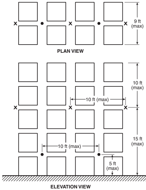
FIGURE 16.6.4(d) Double-Row Rack Sprinkler Layout 9 — Option #1.
