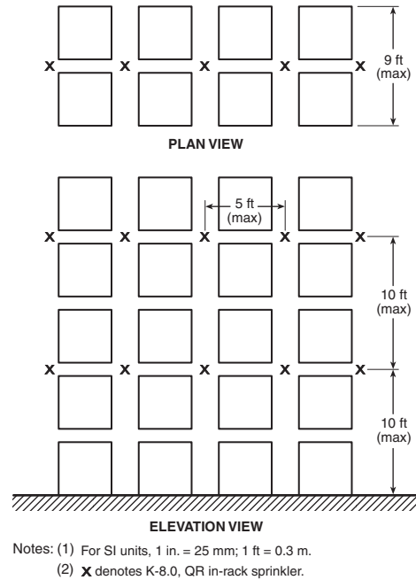
FIGURE 16.6.4(c) Double-Row Rack Sprinkler Layout 8 — Option #2.
