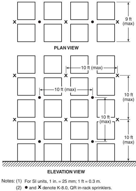
FIGURE 16.6.4(b) Double-Row Rack Sprinkler Layout 8 — Option #1.
