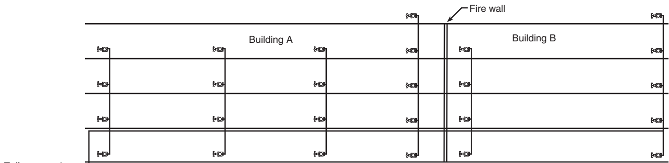
▲ FIGURE A.7.10.1.2.3.1 Common Supply Piping Standpipes Calculated.
