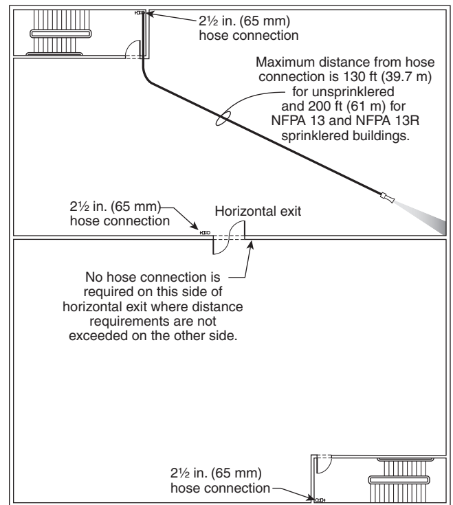
Δ FIGURE A.7.3.2.2.1 Location of Hose Connections at Horizontal Exits and Stairwells.
