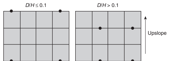
▲ FIGURE A.13.7.4.3.4.5 Spot-Type Detector Spacing for Sloping Ceilings with Beam Pockets. [72: Figure A.17.7.3.2.4.5]
