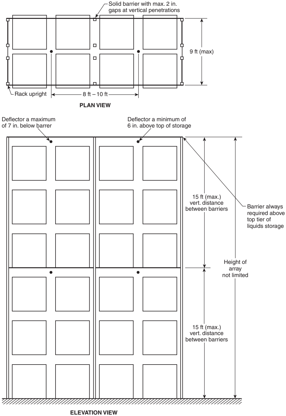
FIGURE 66.16.6.4.1(b) Double-Row Rack Sprinkler Layout for Design Scheme “E.” [30:16.6.4.1(b)]
